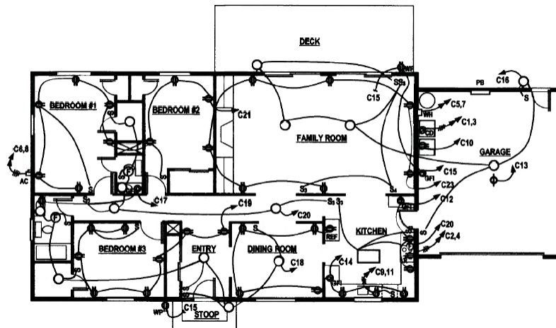
FIGURE 19.15 Circuit layout and numbering for design example.
